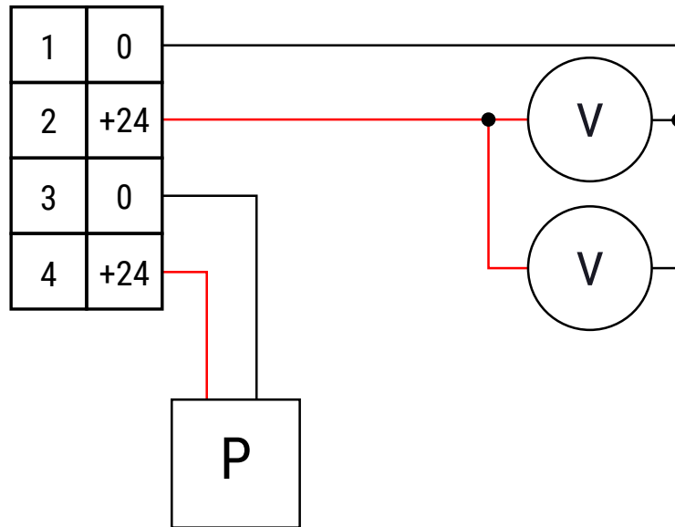
Peltier 50W
